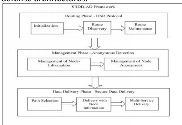
Figure.3.1 Architecture Design
