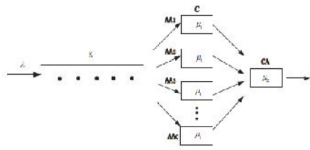
Figure 4.1: Queue Model With Single-Ca/Multi-Aas
