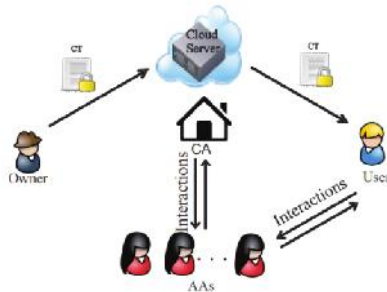
Figure 3.1: Architecture Diagram
