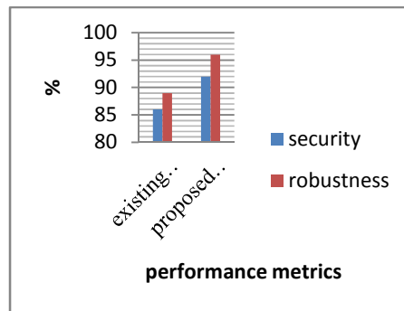
Figure 4.3: Performance Table
